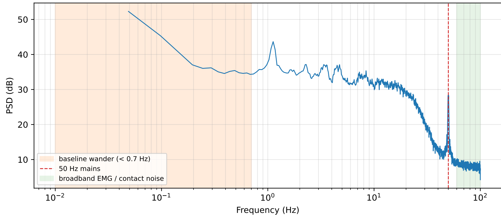
Welch PSD of the raw ECG - identification of the noise sources
